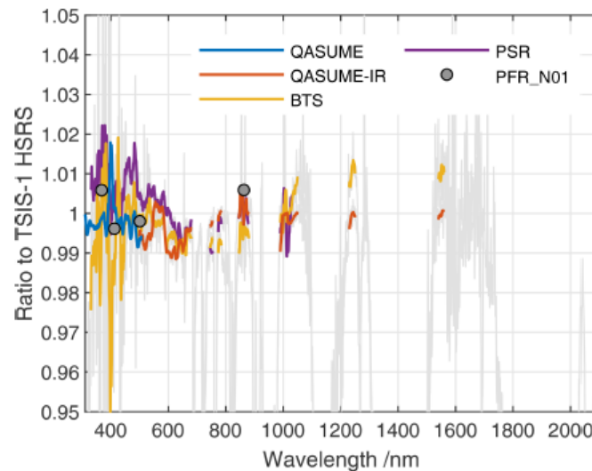
Fig. 3, Spectral ratio of the zero-air-mass-extrapolated ToA solar spectra from QASUME (blue), QASUME-IR (red), the PSR (violet), and the BTS (yellow) relative to the TSIS-1 HSRS convolved with the respective line spread functions of the spectroradiometers. The coloured lines are a 10 nm moving average of the spectral ratios in spectral regions with no or only weak atmospheric trace gas absorption, while the grey line represents the full spectral ratio of the BTS to the TSIS-1 HSRS. The grey circles represent the ratios of the spectral solar irradiances of PFR N01 with the TSIS-1 HSRS convolved with the spectral filter transmissions of PFR N01.
