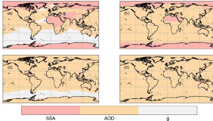
Fig. 6 The largest contributor to the uncertainty in each of the three single scattering properties for four different cases: top of atmosphere (TOA) Direct Aerosol Radiative Forcing (DARF, panel (a)), TOA Direct Aerosol Radiative Effect (DARE, panel (b)), surface DARF (panel (c)) and surface DARE (panel (d)).
